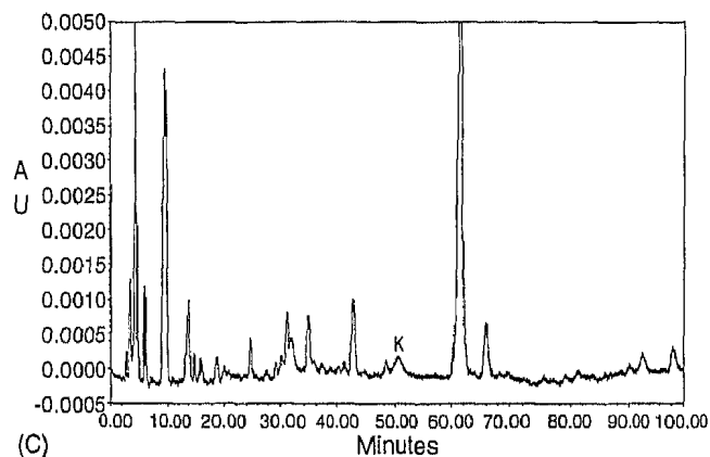
Fig. 4. HPLC chromatograms of (A) cytokinin standards mixture; (B) coconut water extracts; and (C) spiked coconut water extracts by kinetin. Chromatography was performed as described in Table 3.
