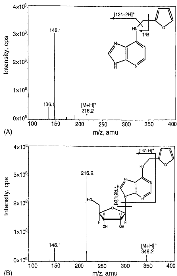
Fig. 1. The positive product ion spectra of (A) kinetin and (B) kinetin riboside, each with the protonated molecule ( [M+H]^+ ) as a precursor ion. (♦) indicates the precursor ion. The chemical structures of the compounds are displayed and their cleavage sites are indicated with arrows pointing to the product ions and their respective m/z .
