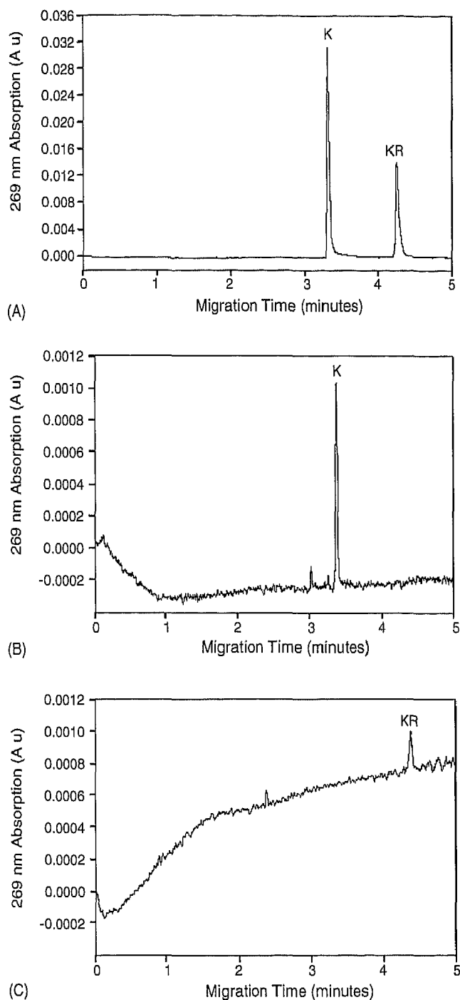
Fig. 6. Electropherograms of (A) kinetin and kinetin riboside standards; (B) putative kinetin chromatographic fraction; and (C) putative kinetin riboside chromatographic fraction. Note: running buffer solution contained 100 mM phosphate ammonium salts (pH 2.5). Other experimental conditions were as described in Section 2.6.
