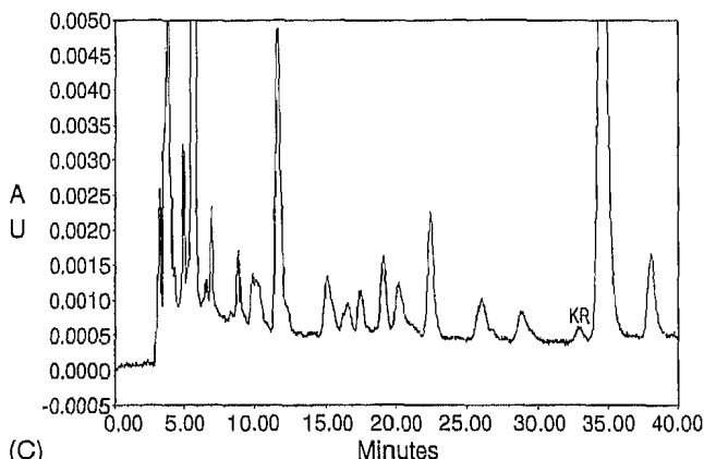
Fig. 5. HPLC chromatograms of (A) kinetin riboside standard; (B) coconut water extracts; and (C) spiked coconut water extracts by kinetin riboside. Chromatography was performed as described in Table 4.
