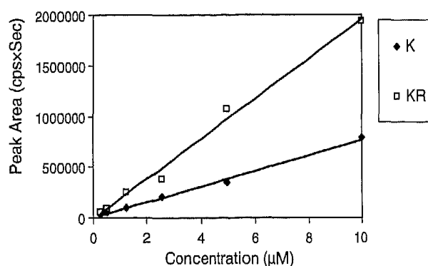
Fig. 2. Standard calibration curves of peak areas against the concentrations for kinetin and kinetin riboside using LC-MS/MS analysis.
