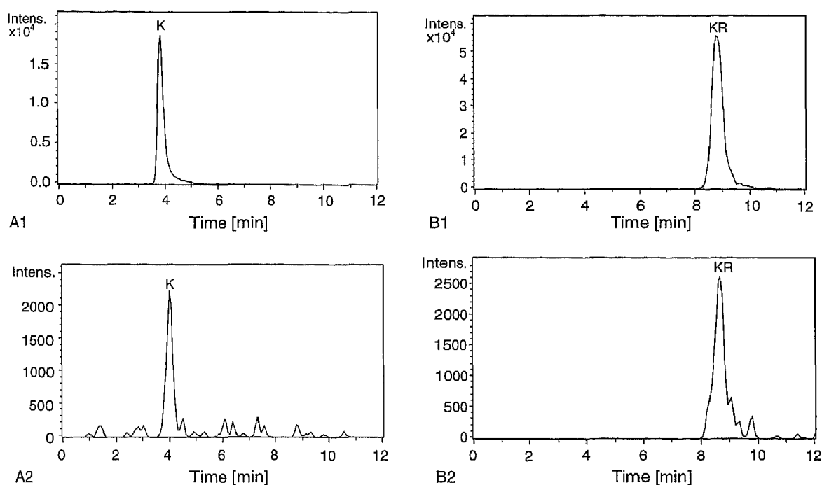
Fig. 3. Representative SRM chromatograms of (A1) kinetin standard; (B1) kinetin riboside standard; (A2) putative kinetin in coconut water extract sample; and (B2) putative kinetin riboside in coconut water extract sample determined by LC–MS/MS method. All other LC parameters and MS conditions were as described in Section 2.4.
